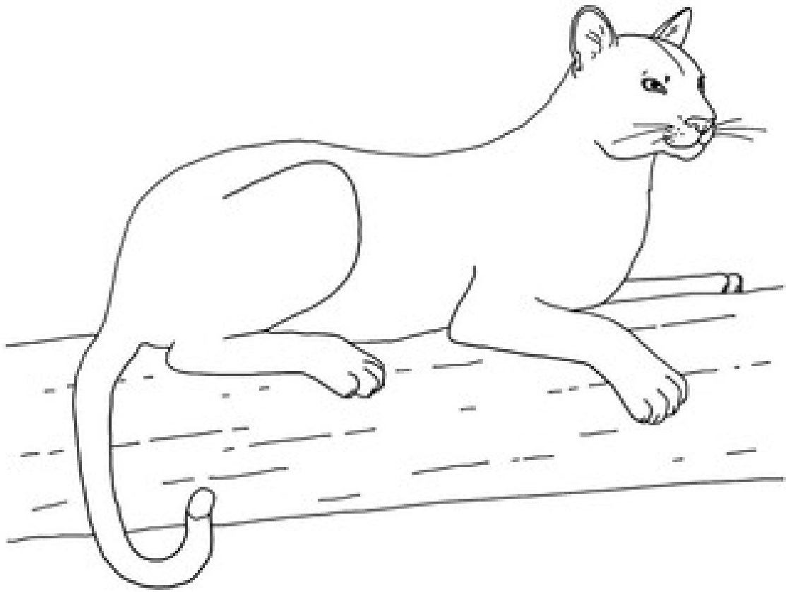
Florida Panther
